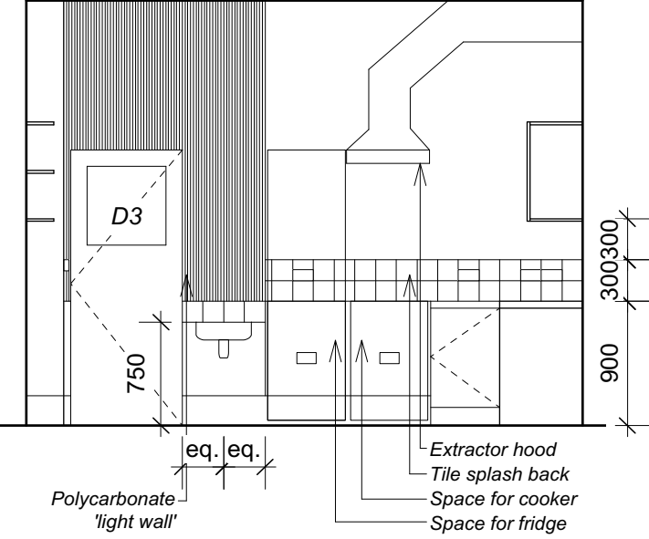
Elevation C
