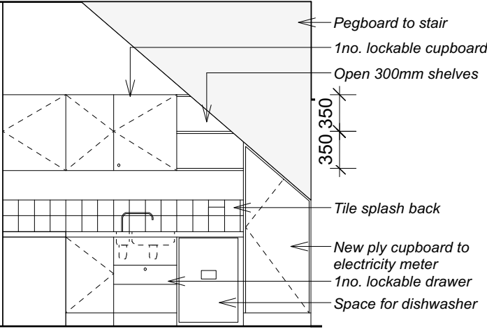
Elevation D
